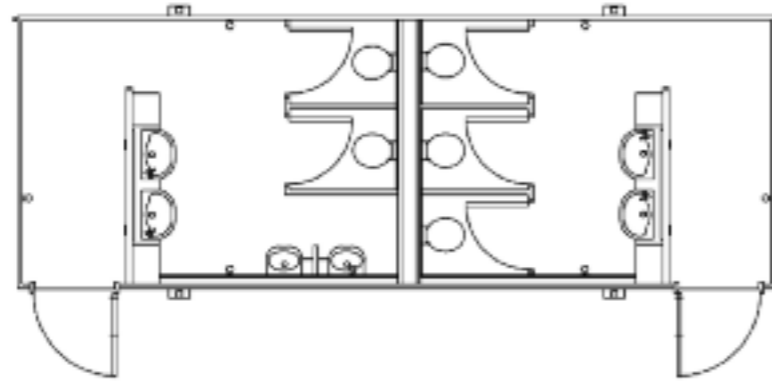
PP282 Male/female Luxe toilet unit 8.64m x 3.27m
