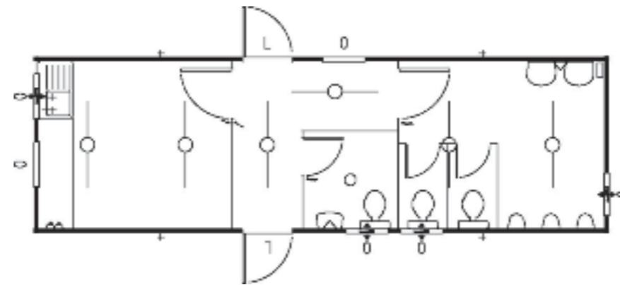
PK342 Pacemaker building with Link corridor Mess/toilet block - floor area 29.60m 2
