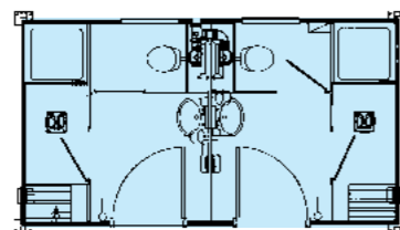
Portaloo 161 (type D) Male/Female toilet/shower unit Mains: 5.08 x 2.90m
