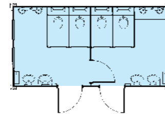
Portaloos 202 (type I) Male/Female toilet unit Mains: 6.08 x 3.27m
