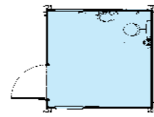
Portaloos 101 (type A) Disabled persons toilet unit Mains: 3.08 x 2.90m
