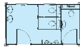
Portaloos 161 (type E) Male/Female toilet unit Mains: 5.08 x 2.90m
