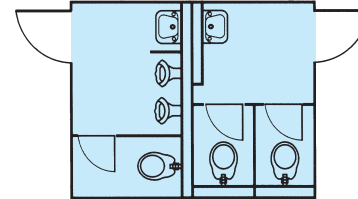
Portaloo 360 Male/Female toilet unit Mains: 3.7m x 3.0m
