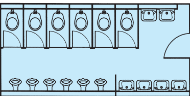
Portaloo 600 Male toilet unit Mains: 6.1m x 3.0m
