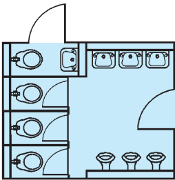
Portaloo 360 Private compartment toilet unit Mains: 3.7m x 3.0m
