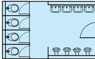
Portaloo 480 Male toilet unit Mains: 4.9m x 3.0m
