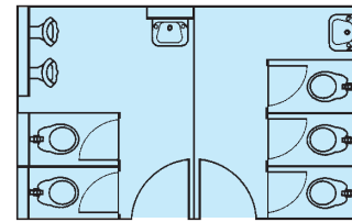
Portaloo 480 Male/Female toilet unit Mains: 4.9m x 3.0m
