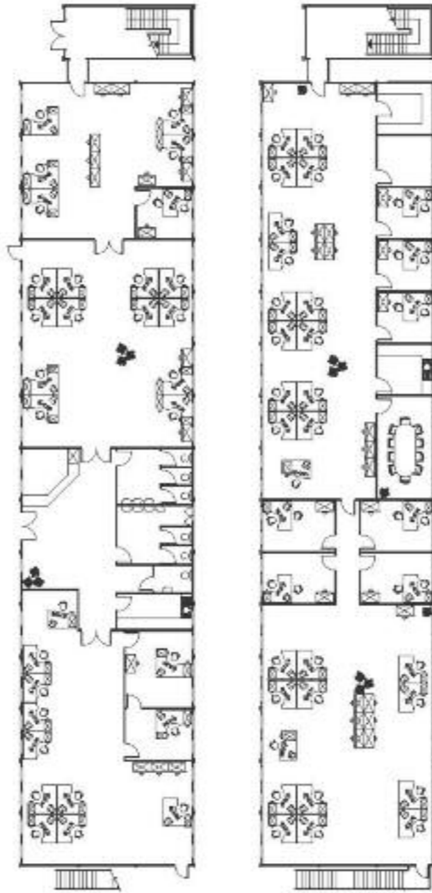
UK093 Two-storey Ultima office complex - total floor area 848.20m 2 (2 x 424.10m 2 )
